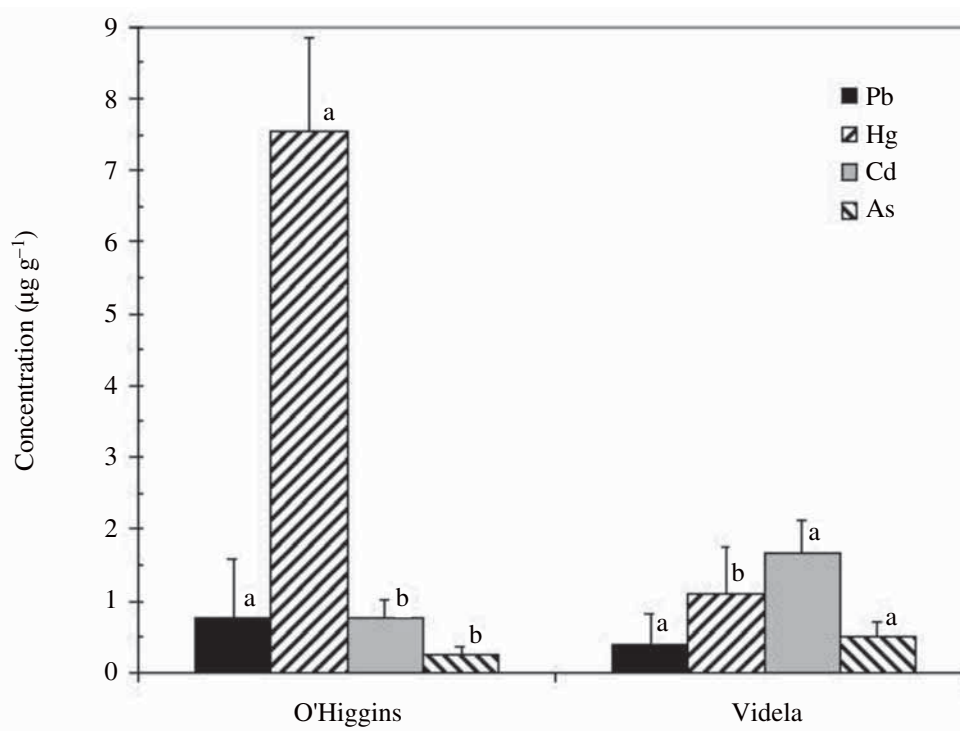
Figure 2. Mean concentrations of trace metals from samples of excrements of Gentoo penguin colonies measured at O'Higgins and Videla, Antarctic Peninsula. Colonies with the same letter for a given element are not significantly different ( P < 0.05 ).
