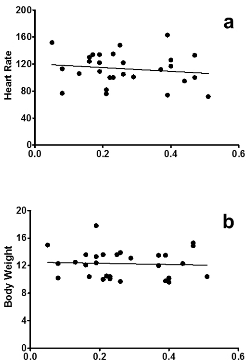
Figure 3. Scatterplots showing non-significant correlation coefficients between the Tei index of myocardial performance and either (a) heart rate (R = 0.1506, P = 0.4346) or (b) body weight (R = 0.0529, P = 0.7822) in healthy Beagles (n = 29). Best-fit lines are shown.
