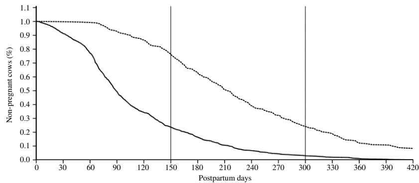
Figure 1. Survival curve showing the percentage of cows with OFC (---) and without OFC (—) remaining open; P < 0.05 .
